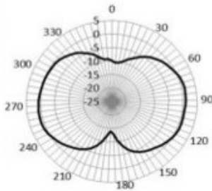
Radiation pattern 690-960 MHz
