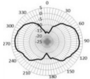
Radiation pattern 2.2- 6 GHz
